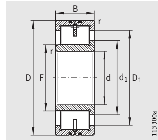
LSL1923
