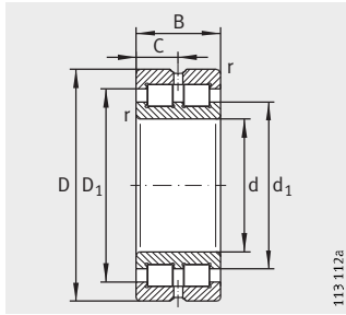
SL0148, SL0149 Festlager
