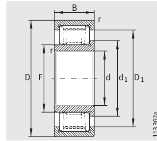
ZSL1923
