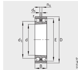
NN30..-AS-K-M-SP Kegel 1:12
