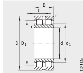
SL0148, SL0149 Festlager
